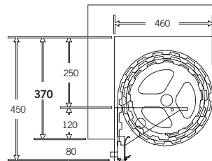
NORMAL HEADROOM Over 2200mm High
